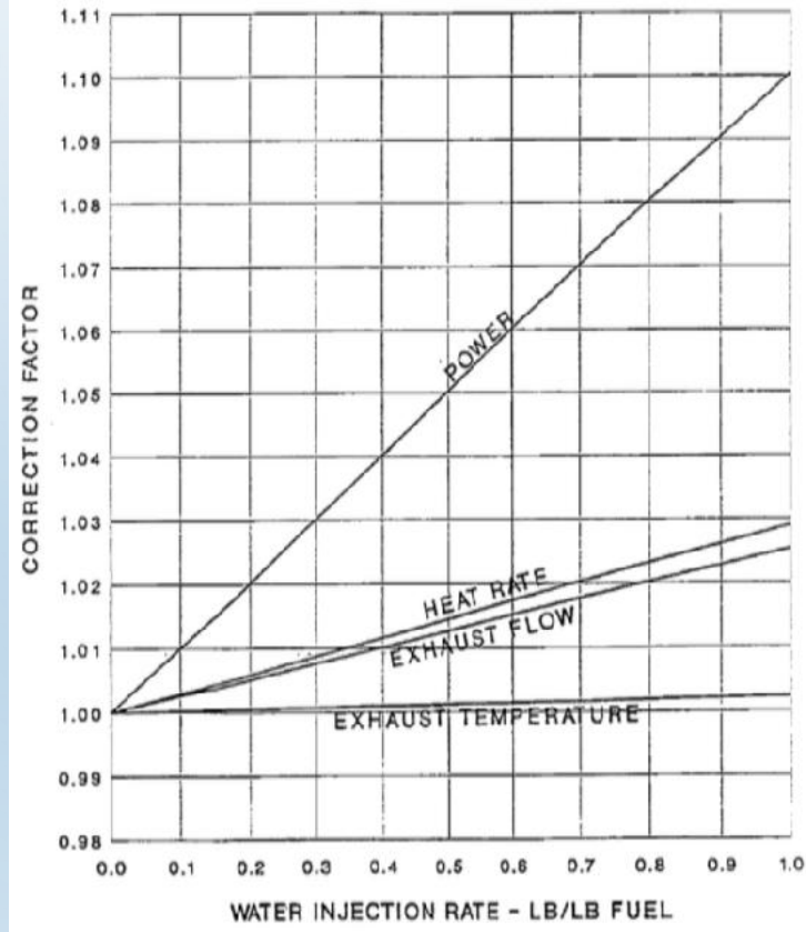
CORRECTION CURVE FOR POWER, HEAT RATE, EXHAUST TEMP & FLOW vs WATER INJECTION No. 2 FUEL OIL FIGURE 7a
